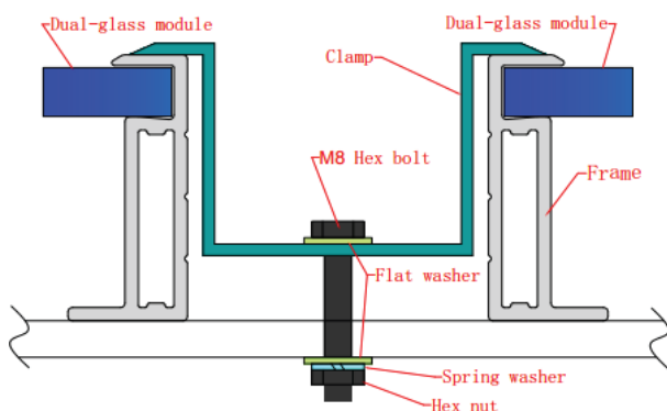
Figure 3 Double-side clamp installation
