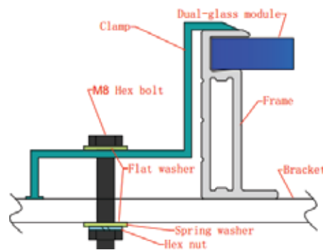
Figure 4 Single-side clamp installation
